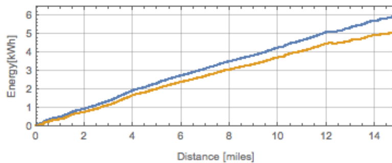
Figure 33. Estimated EV energy consumption with auxiliary loads on (upper curve) and off (lower curve) for the duty cycle from Vallejo and Fairfield-Suisun
