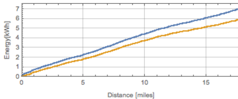
Figure 32. Estimated EV energy consumption with auxiliary loads on (upper curve) and off (lower curve) for the duty cycle from Fairfield-Suisun to Vallejo
